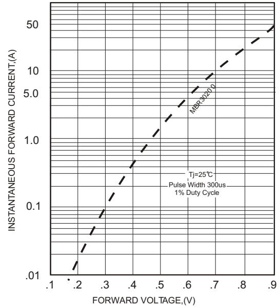
FIG.2-TYPICAL FORWARD CHARACTERISTICS
